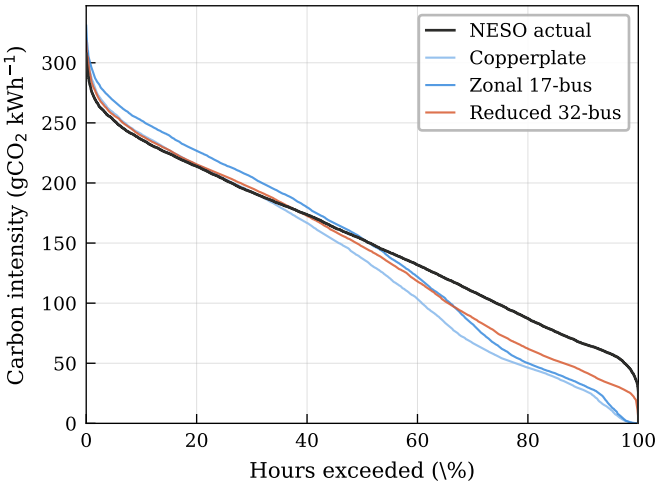
Intensity duration curve — 2023
